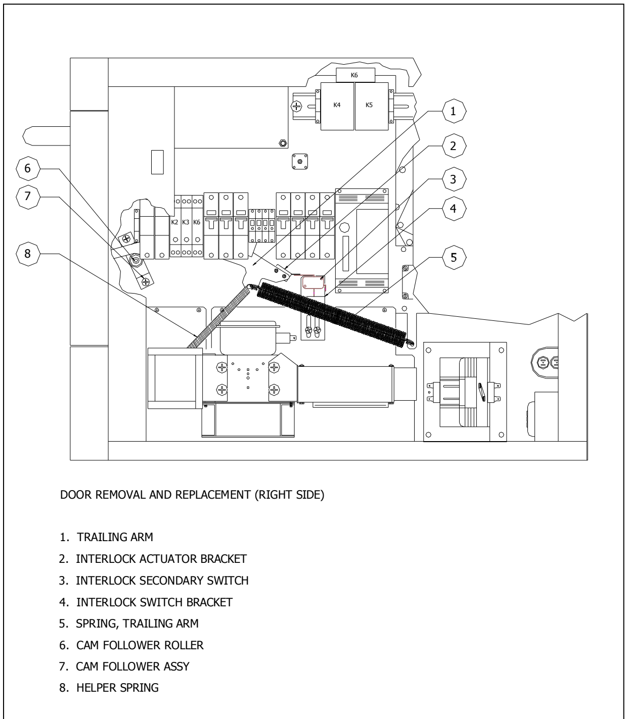
FIGURE 7 – 6b Door Removal and Replacement (Right Side)
